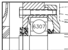
FRONT END DETAIL
